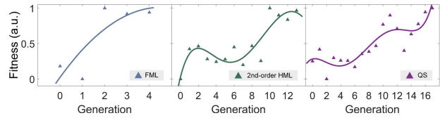
Fig. 4. Normalized average fitness optimization paths of the FML regime, the second-order HML regime, and the QS regime. The triangles indicate the recorded fitness values and the solid lines are the fitted polynomial curves.
